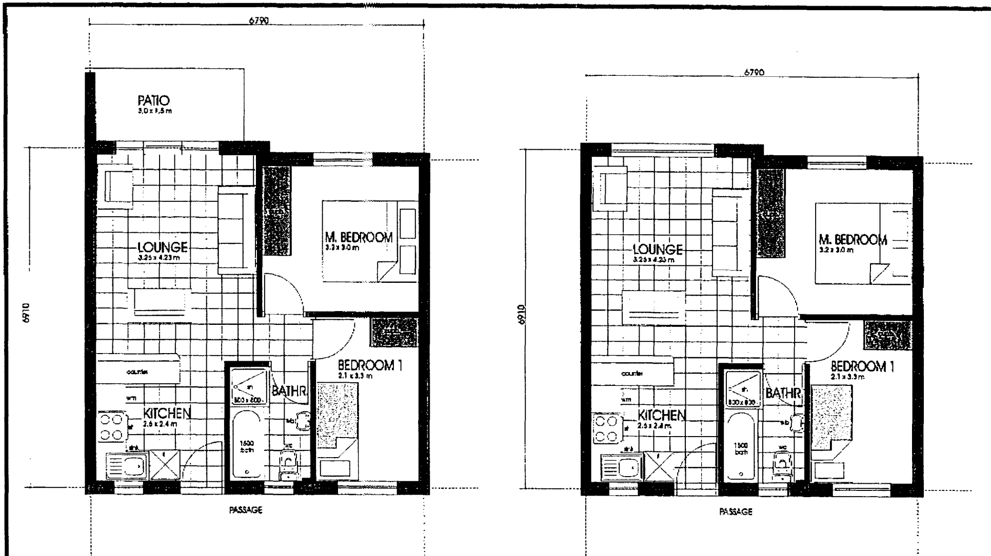
GROUND FLOOR:
